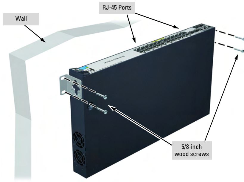
Figure 2-7. Wall Mounting the Switch 2520-24-PoE
