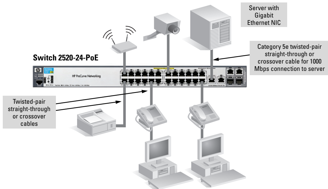
Figure 2-16. Basic desktop configuration
