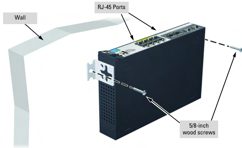
Figure 2-8. Wall Mounting the Switch 2520-8-PoE
