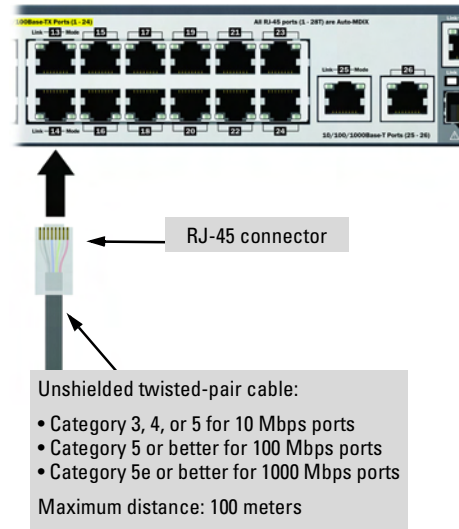
Figure 2-13. Connecting network cables
