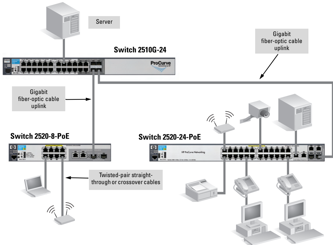
Figure 2-17. Segment network configuration with PoE switches
